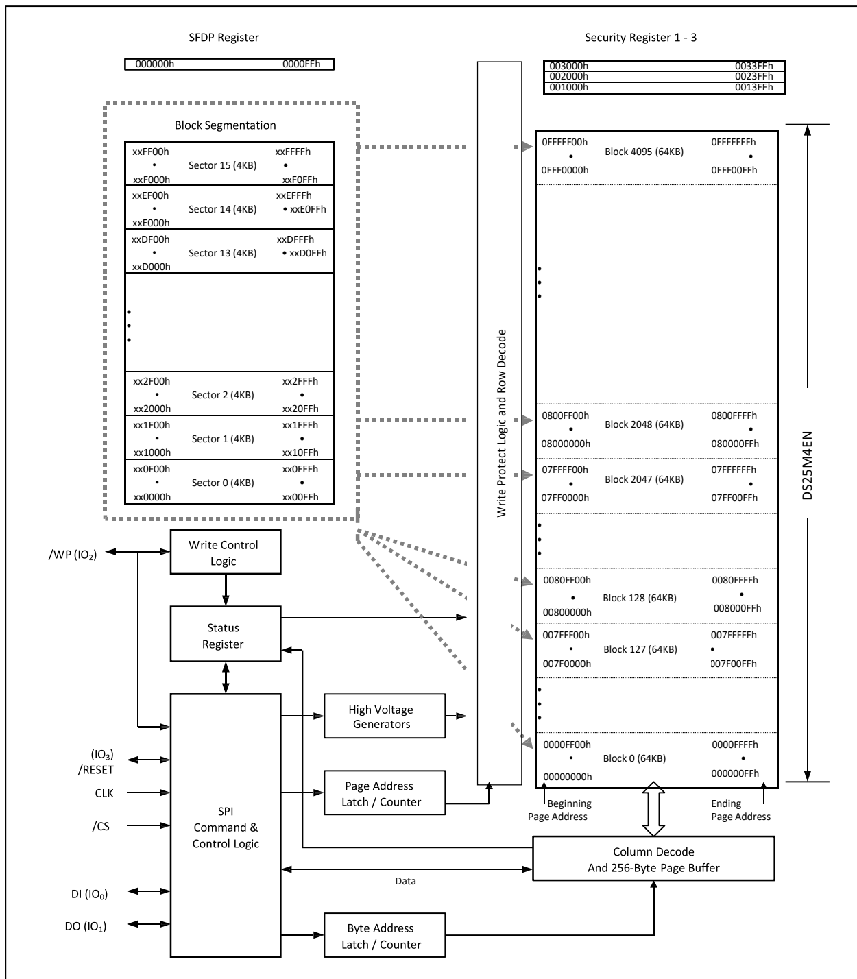
Figure 2. DS25M4EN Serial Flash Memory Block Diagram
