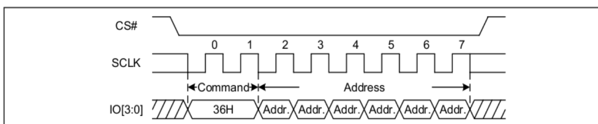
Figure 43b Individual Block/Sector Lock command Sequence Diagram (QPI)
